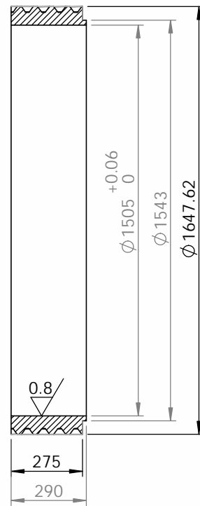
SECTION B-B
